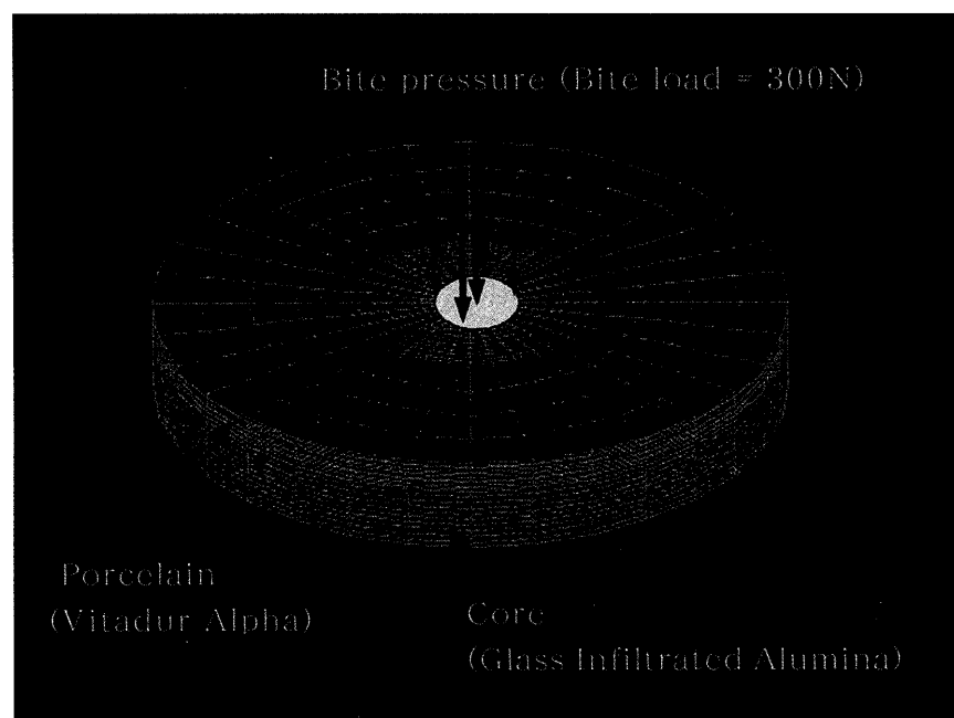
Three-dimensional finite element model with 12453 nodes and 11520 solid elements for a Vitadur Alpha Porcelain / Glass Infiltrated Alumina Core (In-Ceram) bilayered ceramics subjected to a bite load of 300N on a contact surface area of the porcelain. (page 282)
