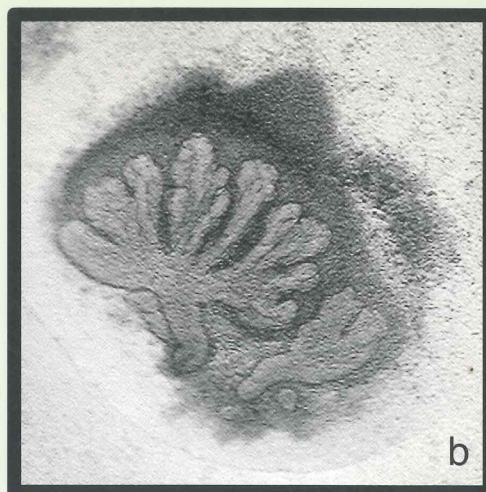
Morphological changes in E13 submandibular gland (SMG) rudiments cultured for 48 hrs without (a) or with MEK inhibitor, 10 \mu M U0126 (b). The branching Morphogenesis of cultured SMG was suppressed by inhibition of Erk activation. (page 119)
