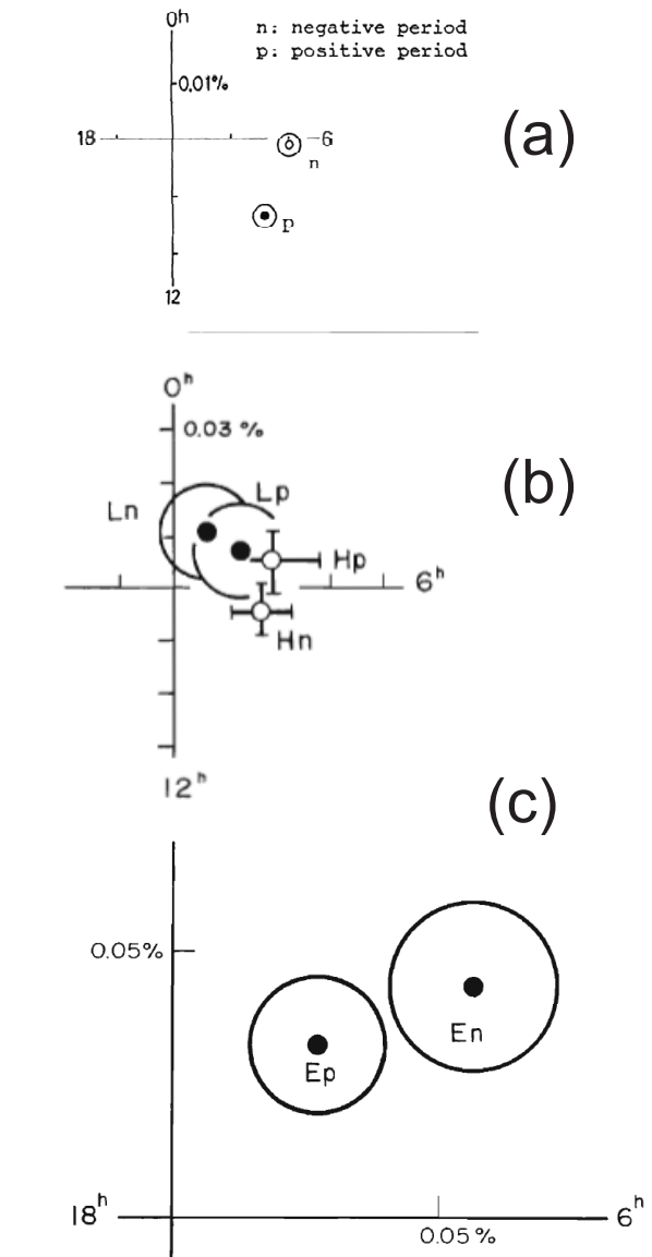
Fig. 11. Polarity dependence of S_iD_1 . (a) Neutron in the N-state (n) (1961–1969) and the P-state (1970–1978). (b) London (L) ( 52^\circ N , 60 m.w.e.) in the N-state (1961–1969; 1981–1982) and the P-state (1970–1978); Hobart (H) ( 43^\circ S , 36 m.w.e.) in the N-state (1958–1969; 1981–1982) and in the P-state (1970–1980). (c) London equatorially pointing telescope (E) (421 GV) in the N-state (1981–1982) and in the P-state (1970–1978).
