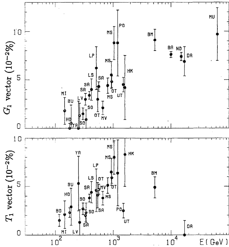
Fig. 17. Energy dependencies of the amplitude GD_1 (0 hr) and TD_1 (6 hr) derived from the observed S_i D_1 's whose phases are shown in Fig. 12 (Ref. 3). The symbols are the same as in Fig. 12. The amplitude for \lambda \neq 0^\circ is converted into that at the equator by multiplying a provisional correction factor 1/\cos \lambda , although its latitude dependence cannot be exactly expressed by \cos \lambda as it contains the north-south asymmetric term ( \sin \lambda ).
