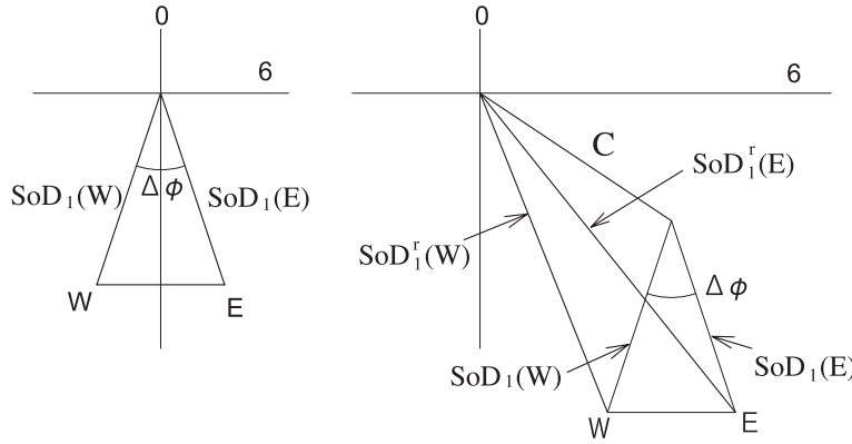
Fig. 1. Elimination of SS_i D by east- and west-ward CR telescopes with the same zenith angle (Elliot, 1952).
