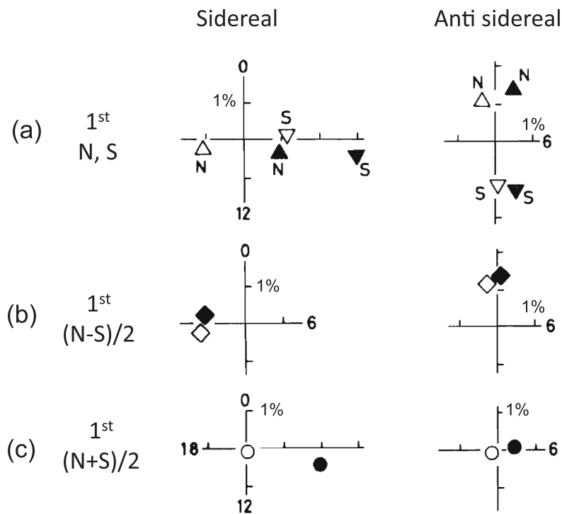
Fig. 9. The elimination of SS_iA from S_i D_1^f by the modified CSSA method, applied to the conjugate S_i D_1^f(N) and S_i D_1^f(S) artificially produced by averaging, respectively, almost all the northern and southern neutron monitor data (Nagashima et al. , 1983a, 1984). Black triangles, observed total vectors; open triangles, expected spurious; black circle, corrected vector; open circle, resulting spurious.
