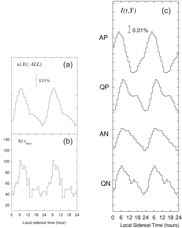
Fig. 20. (a) The average of yearly S_iD(t_{s_i}) 's of neutron intensities observed at 74 stations in the period of 1960–2000. (b) Histogram of the maximum phase of yearly S_iD(t_{s_i}) 's. (c) The modulation patterns of S_iD(t_{s_i}) .
