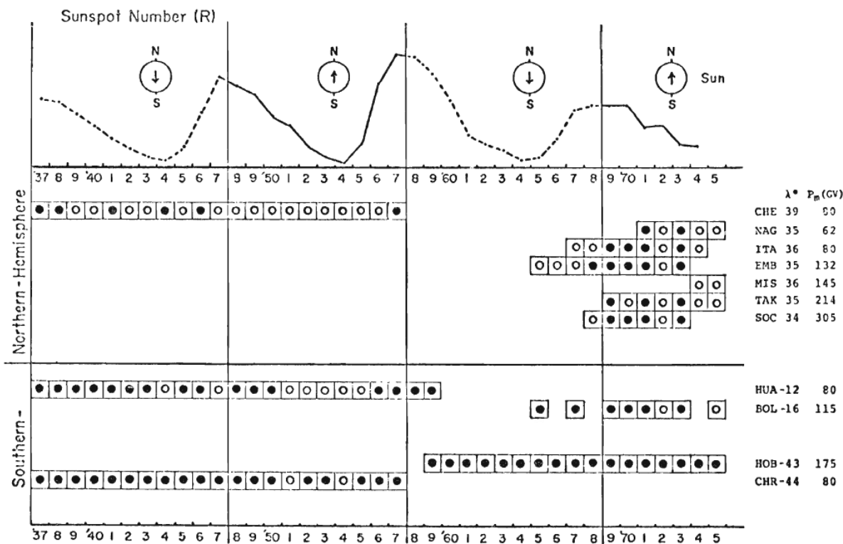
Fig. 7. Time series of phase of \text{SiD}_1^0 without CSSA (Nagashima and Mori, 1976). Solid circle: Morning side (0–12 hr); Open circle: Evening side (12–24 hr); NAG, ITA, MIS and TAK (Ichinose and Murakami, 1976); EMB, SOC and BOL (Swinson, 1976); HOB (Humble and Fenton, 1975; Fenton and Fenton, 1976); CHE, HUA and CHR (Lange and Forbush, 1948, 1957; Beach and Forbush, 1961).
