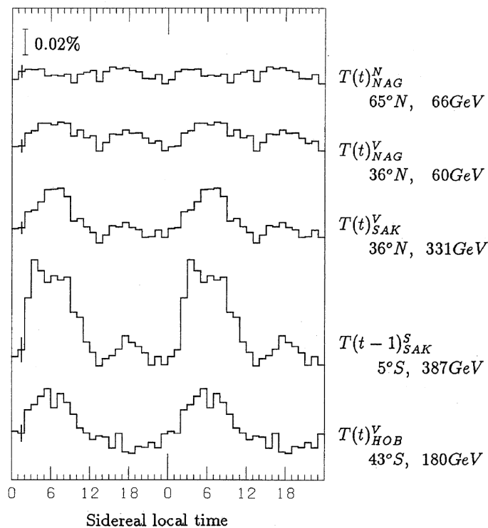
Fig. 16. T(t_{s_i}) due to TA obtained according to the preceding procedure shown in Fig. 15.
