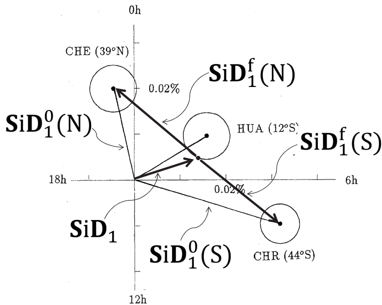
Fig. 6. \text{SiD}_1 's with the error circles observed with the ion chambers at Cheltenham ( \lambda = 39^\circ\text{N} ; \phi = 283^\circ\text{E} ; E_m = 67 GeV) and Christchurch ( 44^\circ\text{S} ; 173^\circ\text{E} ; 67 GeV) during 1937–1958 and at Huancayo ( 12^\circ\text{S} ; 285^\circ\text{E} ; 62 GeV) during 1936–1959, cited from Nagashima and Mori (1976). These results were derived from the data published by Lange and Forbush (1948, 1957) and Beach and Forbush (1961).
