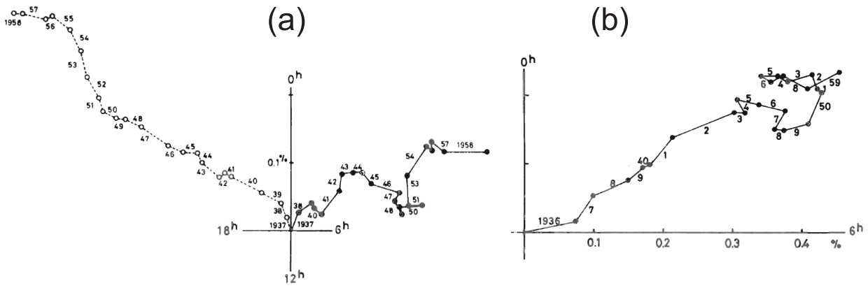
Fig. 8. Summation diagrams \Sigma S_i D_1^f (on the right) and 2\Sigma S_i D_1^f(N) in Fig. 8(a) and of the yearly vectors, and \Sigma S_i D_1^f(HUA) in Fig. 8(b), of the yearly vectors in Fig. 6.
