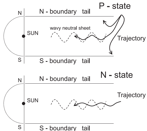
Fig. 26. Cosmic-Ray-Lens Effect of HMS which focuses CRs along the direction of the neutral sheet of HMS. Arrowed curves express the CR trajectories in P- and N-states. Dashed line is the wavy neutral sheet.
